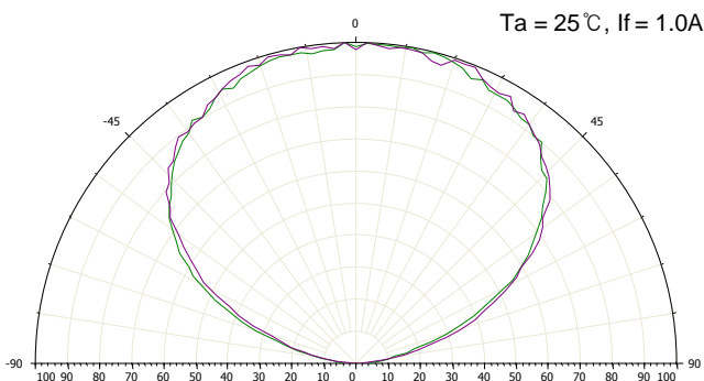
■ Radiation Characteristics
